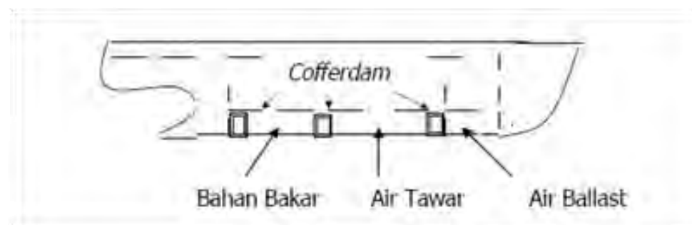
Gambar 33. Cofferdam
