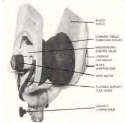
Line hauler
