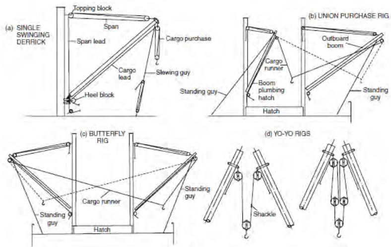
FIGURE 24.2 Derrick rigs
