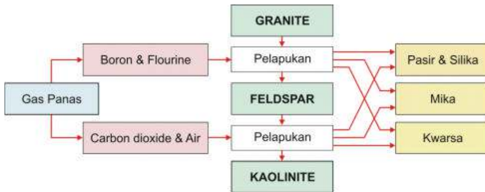
Gambar 6.1. Proses pelapukan batuan granit. (sumber: Frank Hammer and Janet Hammer).
