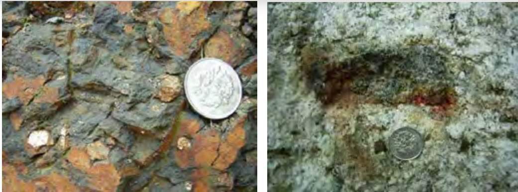
Gambar1.87. Hornblende hornfels facies
