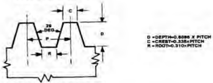
29-DEG WORM SCREW THREAD (BROWN AND SHARPE)
