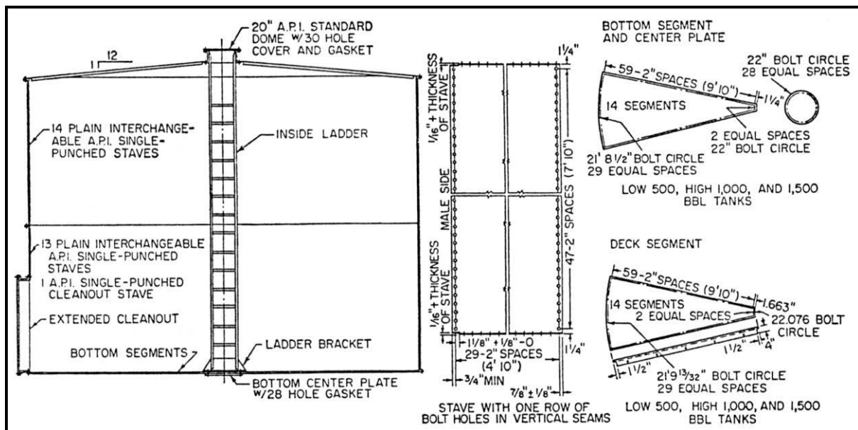
Gambar 8.23. Penampang Storage Tank Jenis Bolted-Steel Tank
