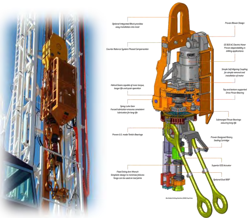
Gambar 4.23. Top Drive
