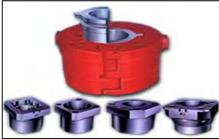
Gambar 4.16. Master Bushing tipe split
