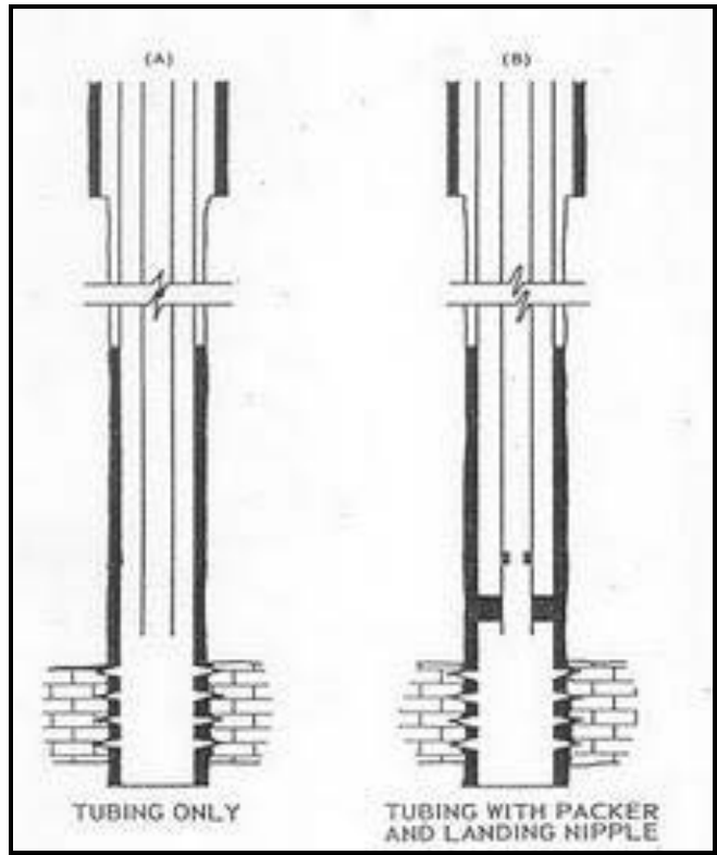
Gambar 6.2. Single Completion
