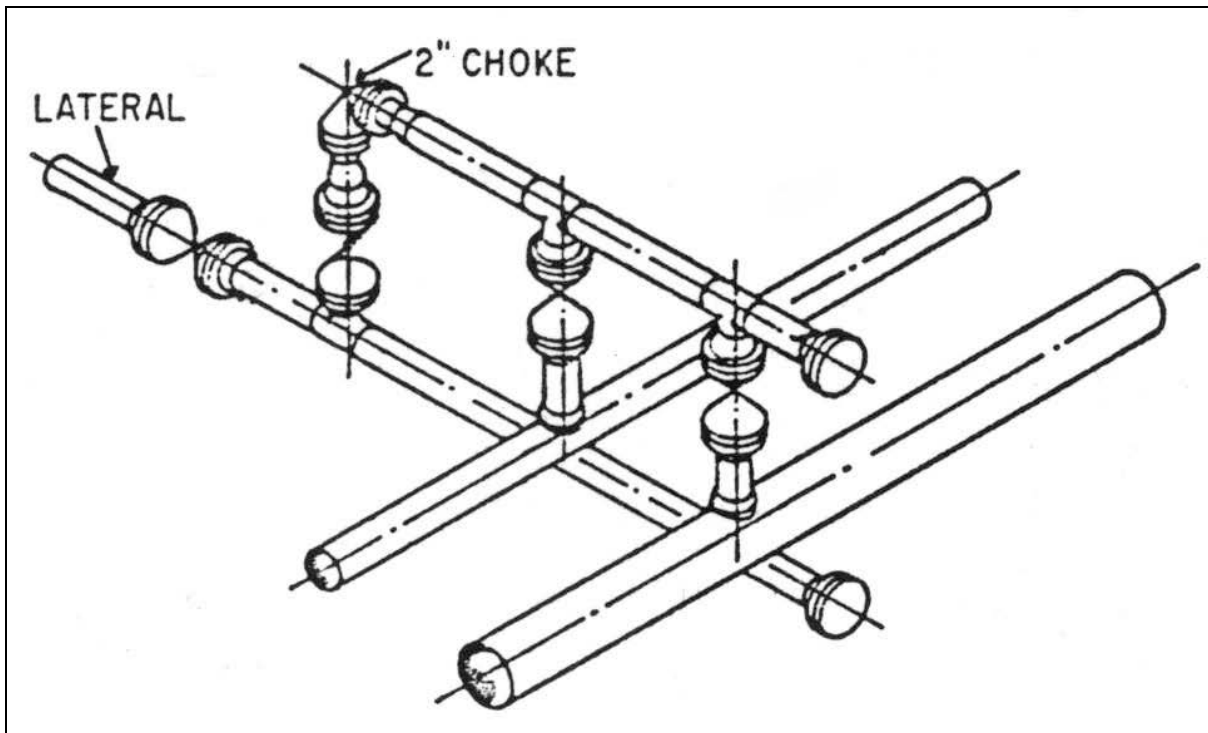
Gambar 8.14. Manifold
