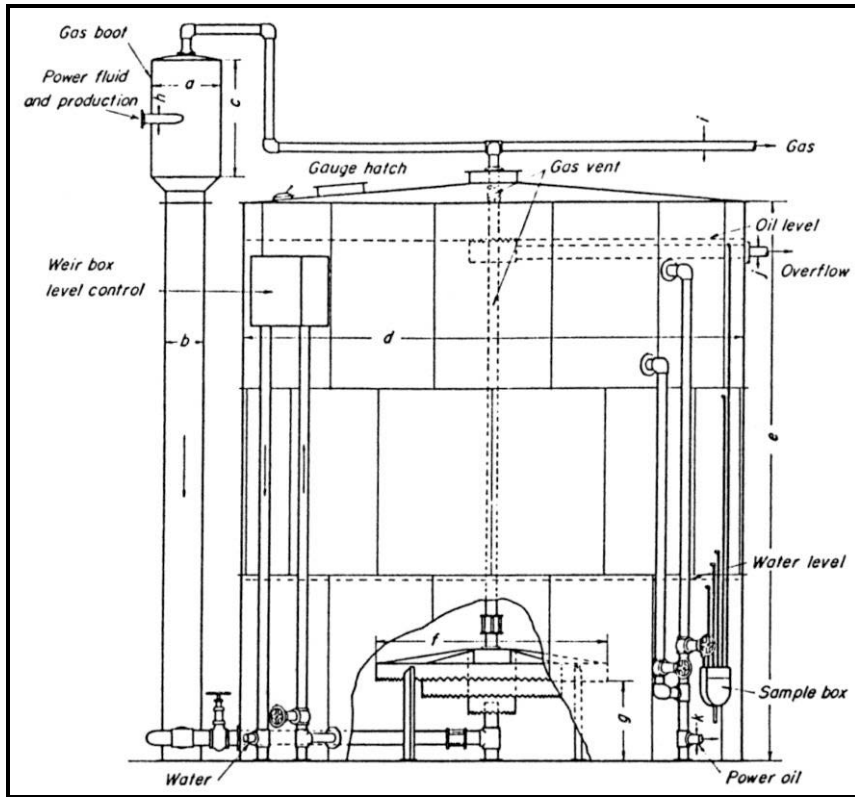
Gambar 8.20. Wash Tank
