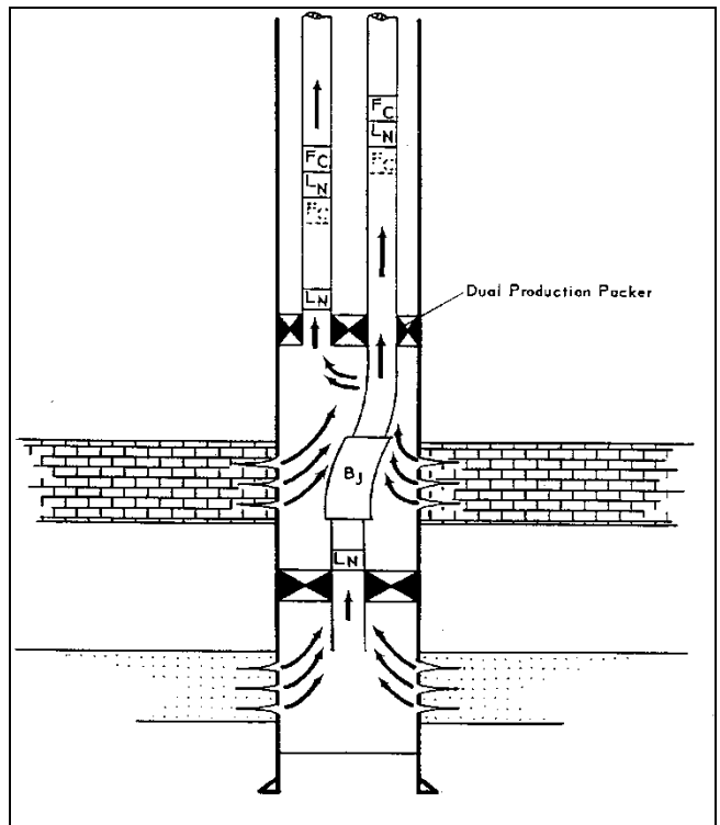
Gambar 6.3. Multiple Completion
