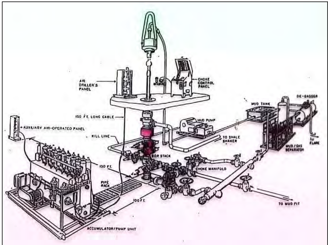
Gambar 4.37. BOP System
