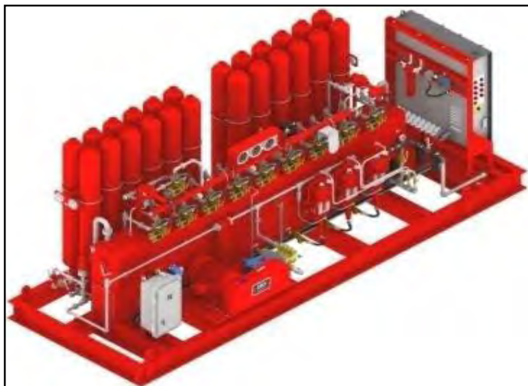
Gambar 4.43. Accumulator Unit
