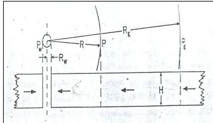
Gambar 8.3. Aliran Radial
