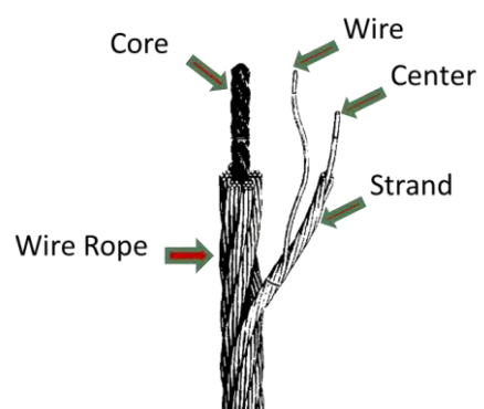
Gambar 4.9. Drilling Line
