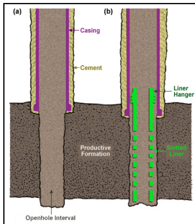
Gambar 6.1. Open Hole Completion
