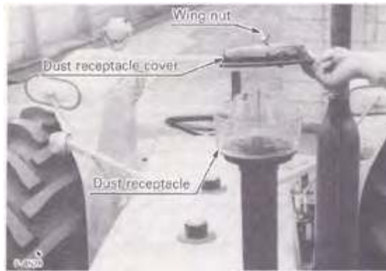
Gambar 45. Pra-penyaring (Pre-cleaner)
