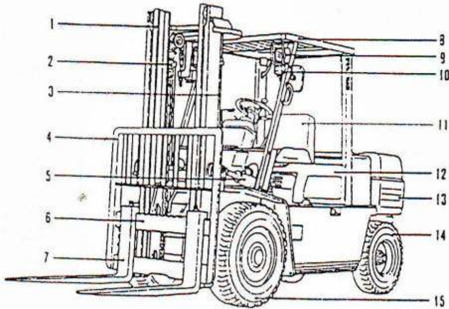
Gambar 5.33 bagian-bagian Forklift
