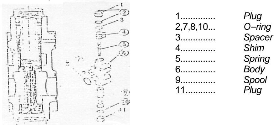
Gambar 4.188 Relief Valve
