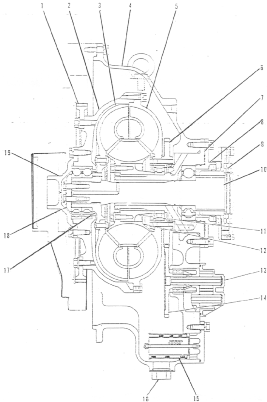
Gambar 4.178 Torque Converter Single Phase (Potongan)
