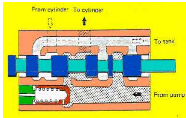
Gambar 4.126 Katup pengontrol arah aliran (directional control valve)
