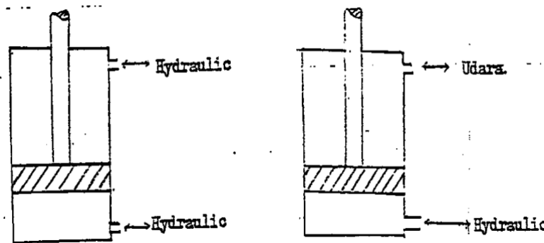
Gambar 4.139 Double acting & single acting cylinders
