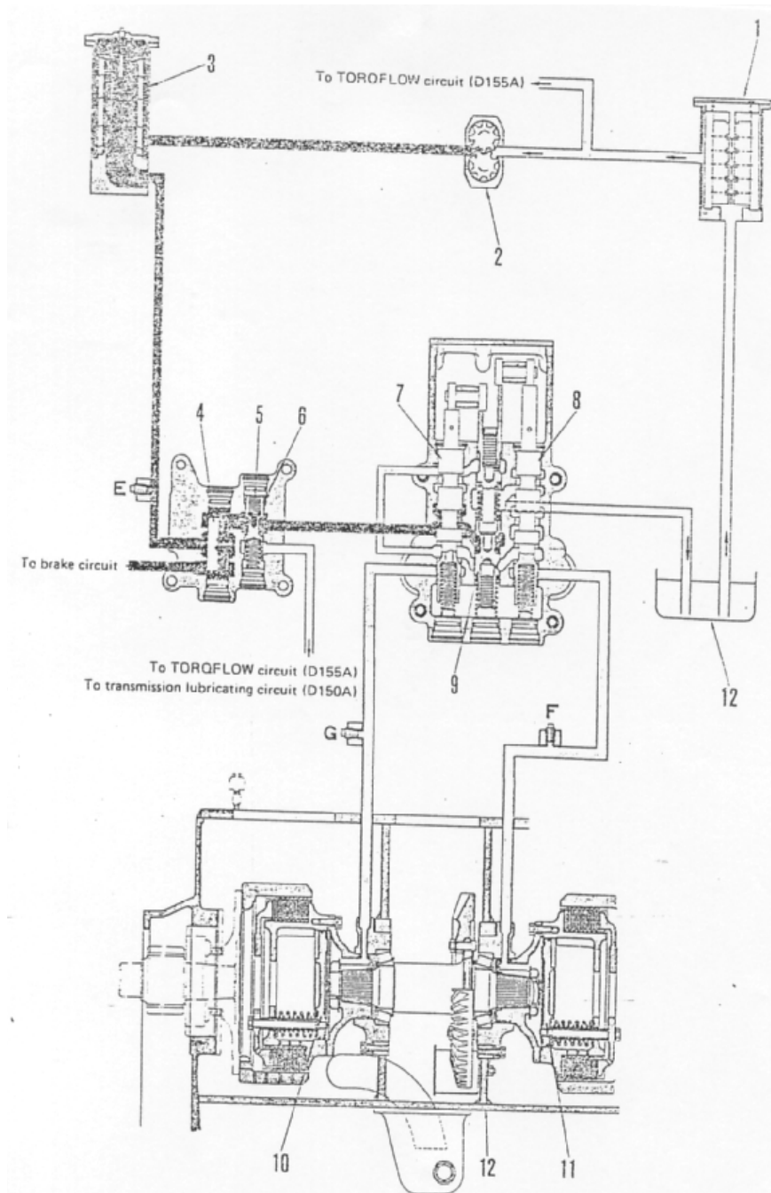
Gambar 4.129 Sirkuit Steering Clutch D150, 155-1
