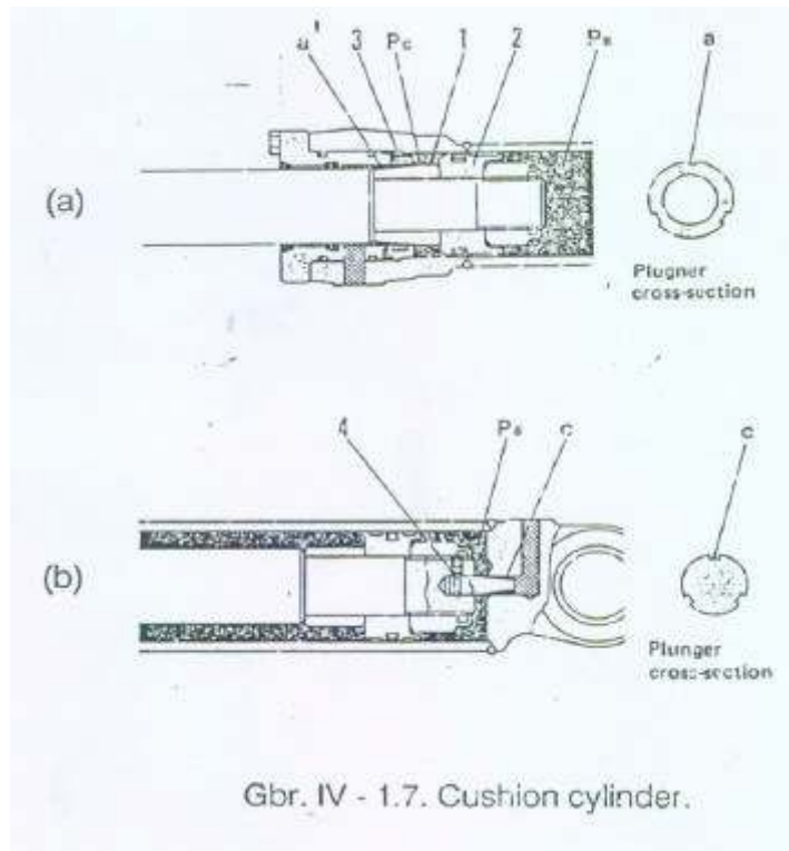
Gambar 4.151 Cushion Cylinder
