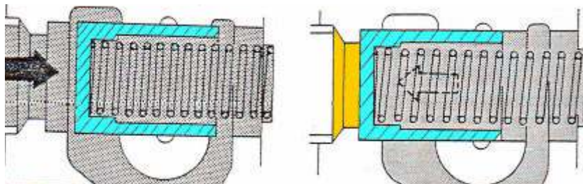
Gambar 4.114 Prinsip kerja make up valve
