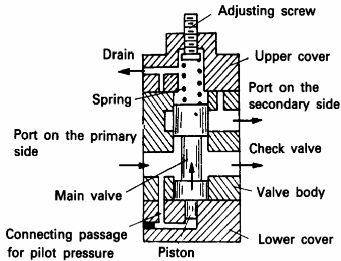
Pressure Sequence Valve
