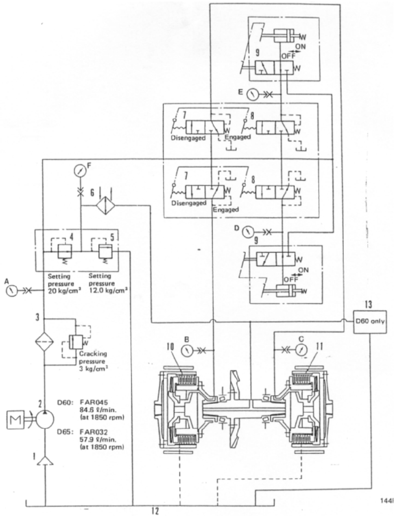
Gambar 4.126 Sircuit diagram D60, 65-7, 8
