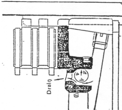
Gambar 4.211 Ball Check valve : Clutch Dis—Engaged
