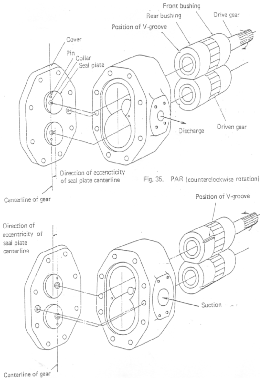
Gambar 4.74 Gear Pump type PAL, R028 – 0250 secara Assembly Drawing
