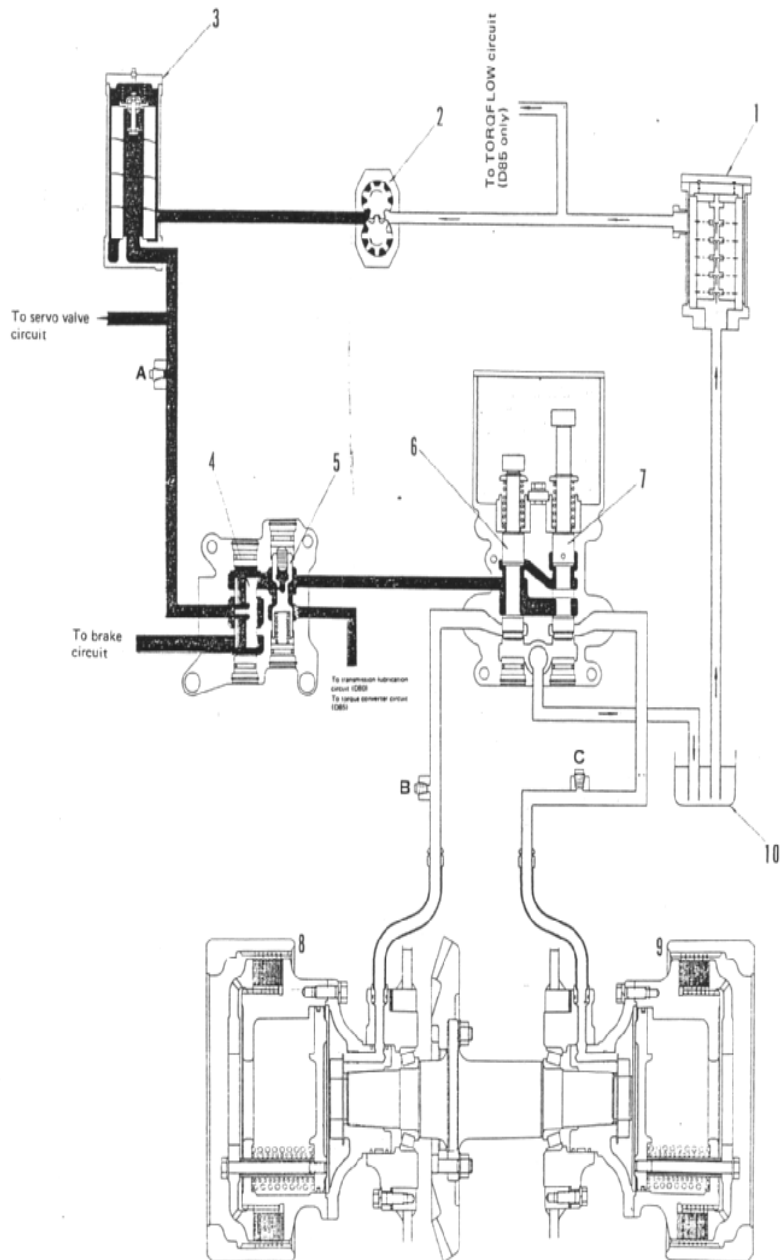
Gambar 4.128 Sirkuit Steering Clutch D80,85-18
