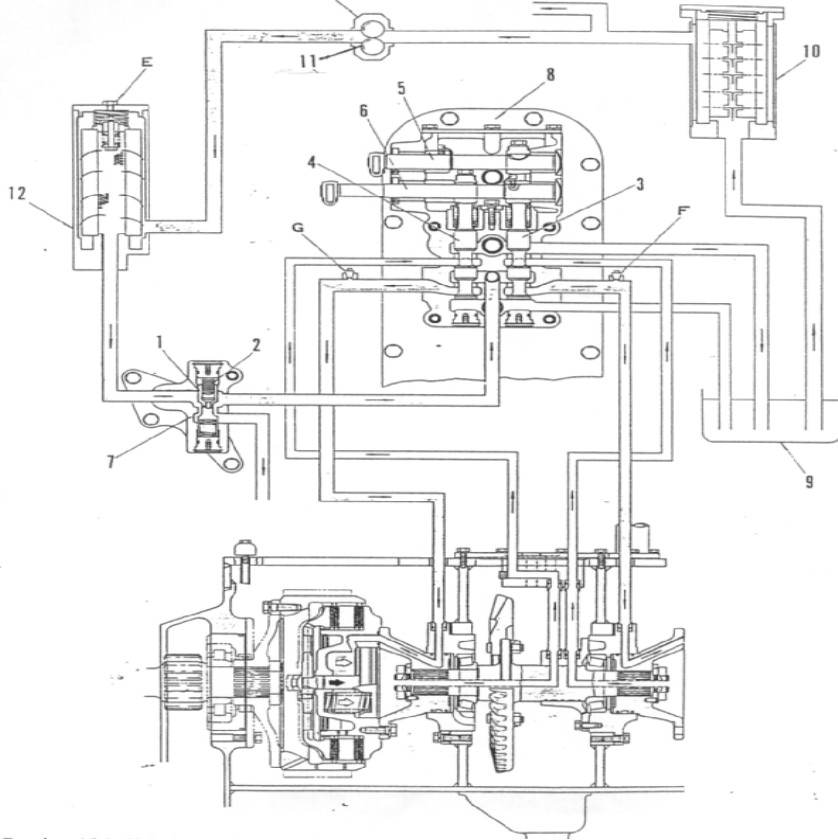
Gambar 4.135 sirkuit Seering Clutch D 80,85-12
