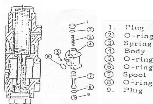
Gambar 4.189 Regulator Valve
