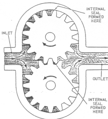
Gambar 4.70 External Gear Pump
