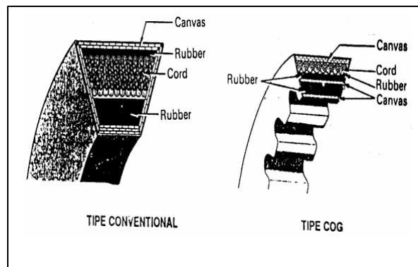
Gambar 4.29. V belt
