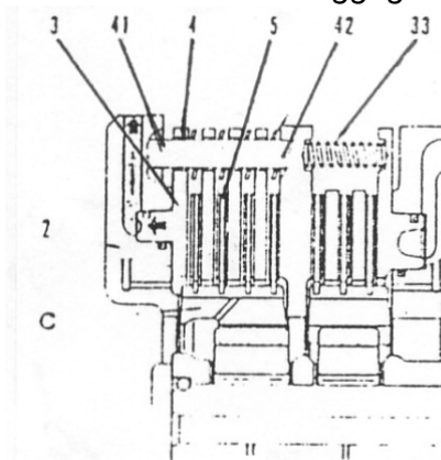
Gambar 4.205 Dis-Enggague
