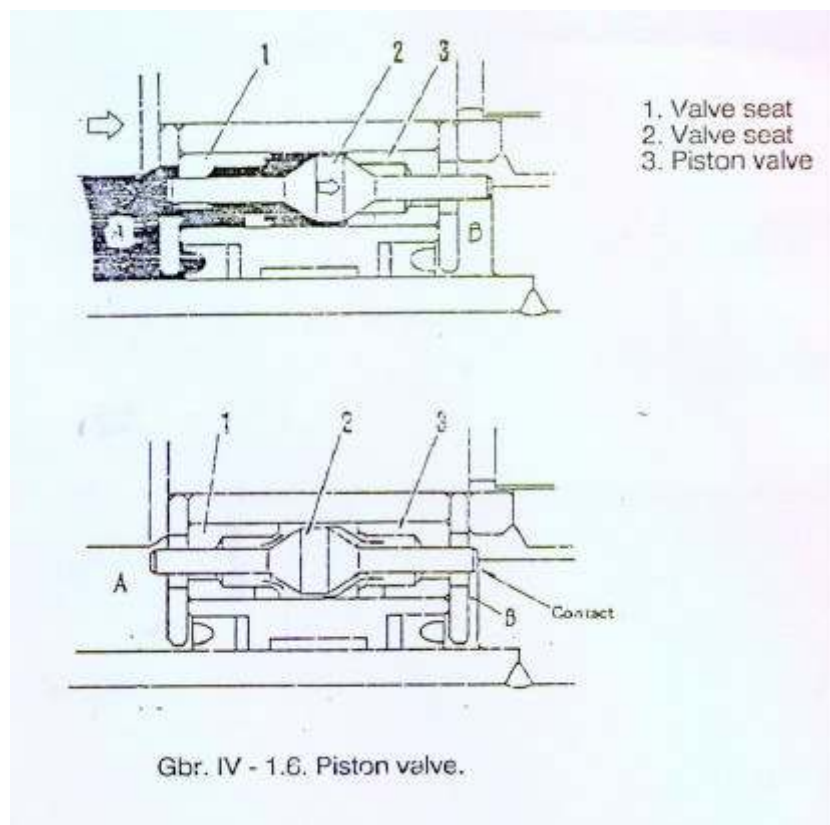
Gambar 4.150 Piston Valve
