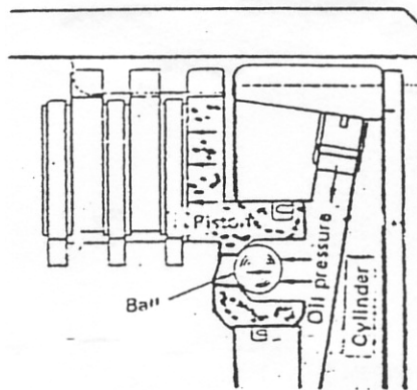
Gambar 4.210 Ball Check Valve : Clutch Engaged
