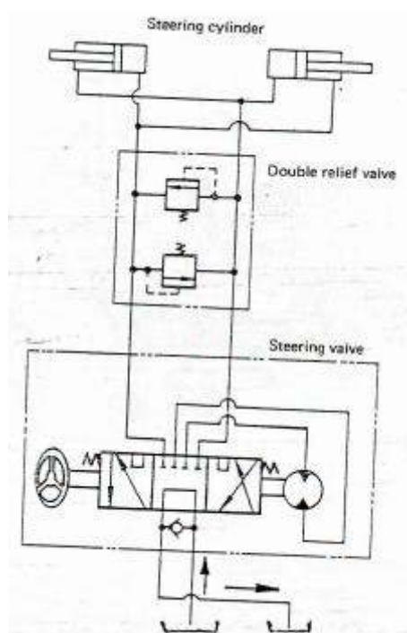
Gambar 4.132 (b) Simbul orbitroll valve
