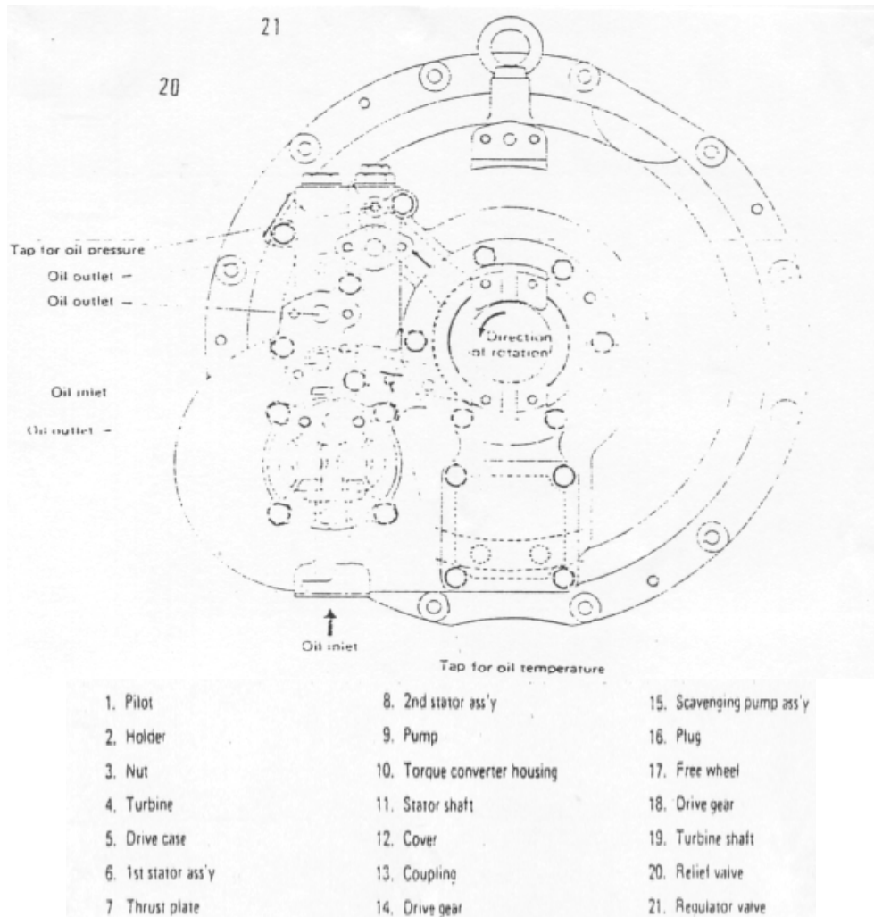
Gambar 4.184 Torque Converter Three Phase (Pandangan Depan)
