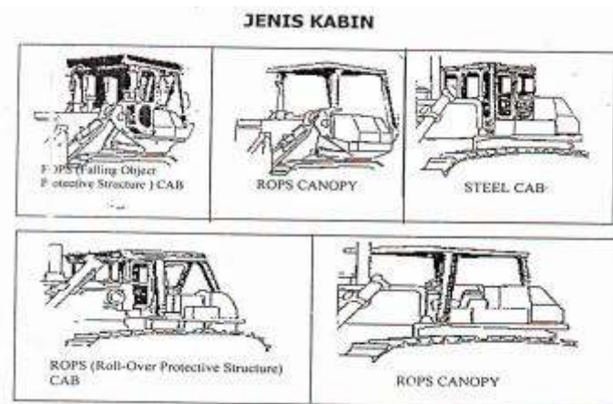
Gambar 5.29 Jenis kabin Doser Shovel
