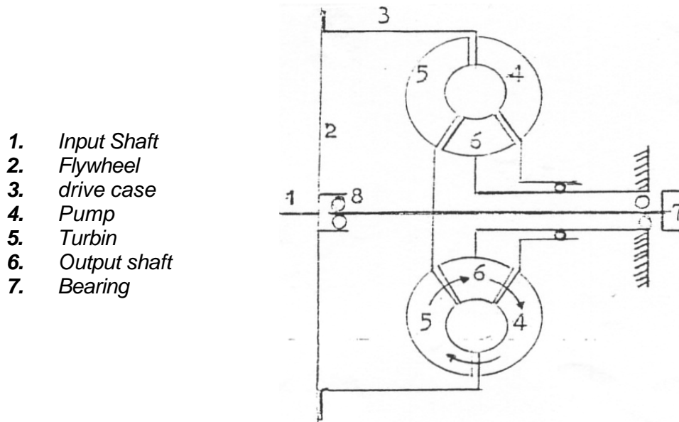
Gambar 4.176 Prinsip kerja torque converter
