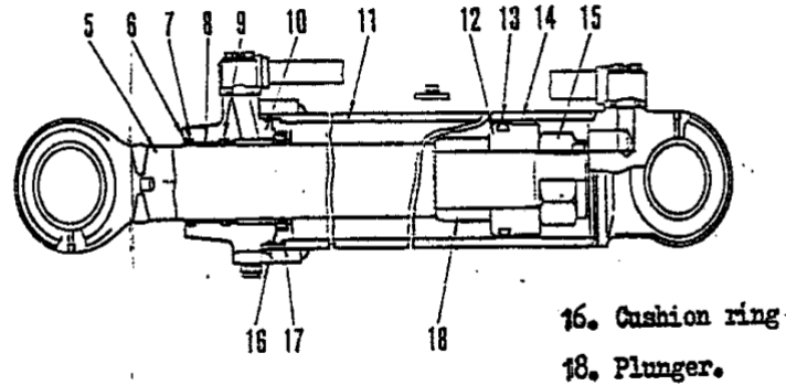
Boom cylinder
