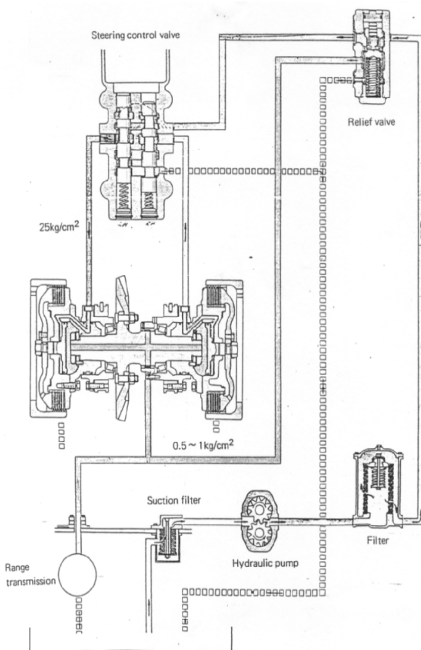
Gambar 4.140. Skema hidrolik Steering Control Valve
