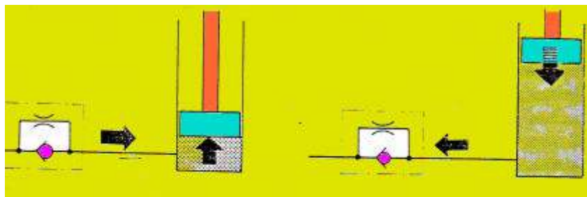
Gambar 4.112 Simbul kerja throttle valve
