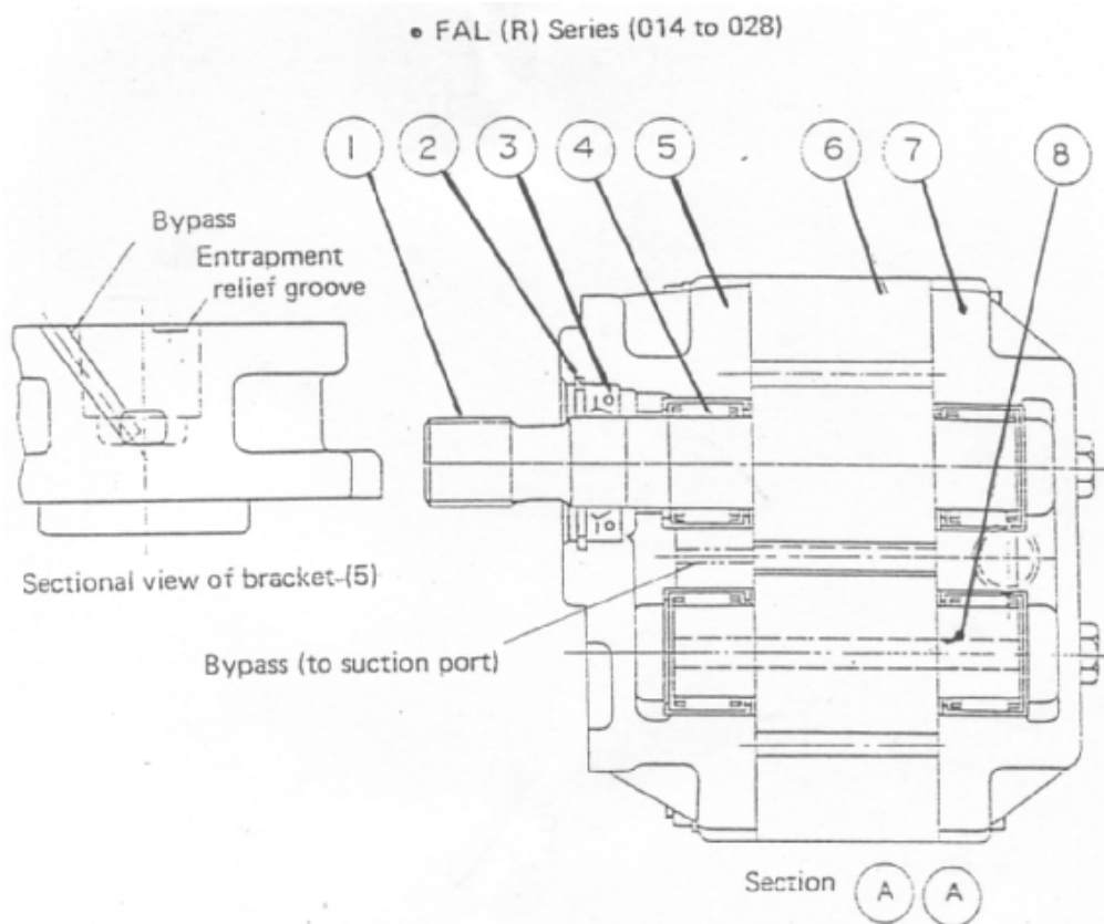
Gambar 4.71 Fixed Side Plate Type Gear Pump
