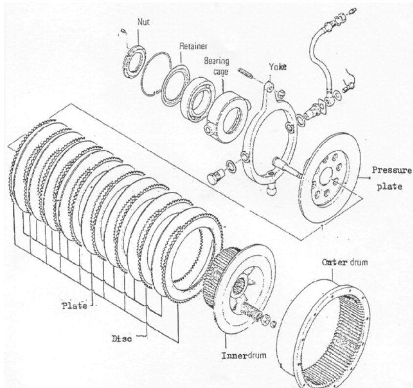
Gambar 4.116 Komponen Steering Cluth mechanical
