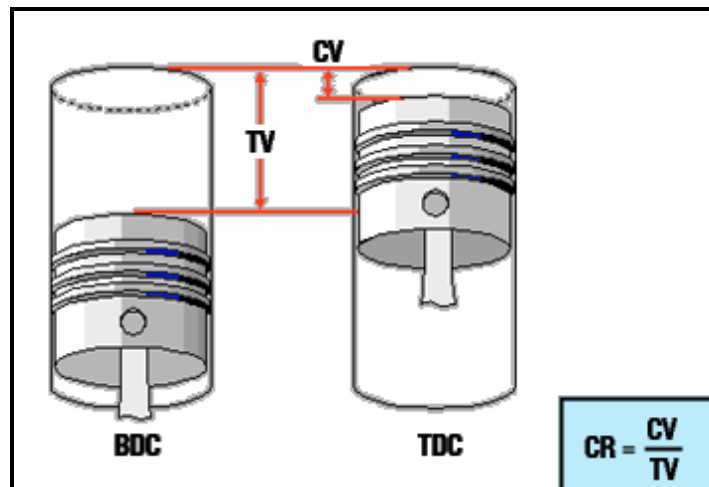
Gambar 4.5 Gambar Compression Ratio
