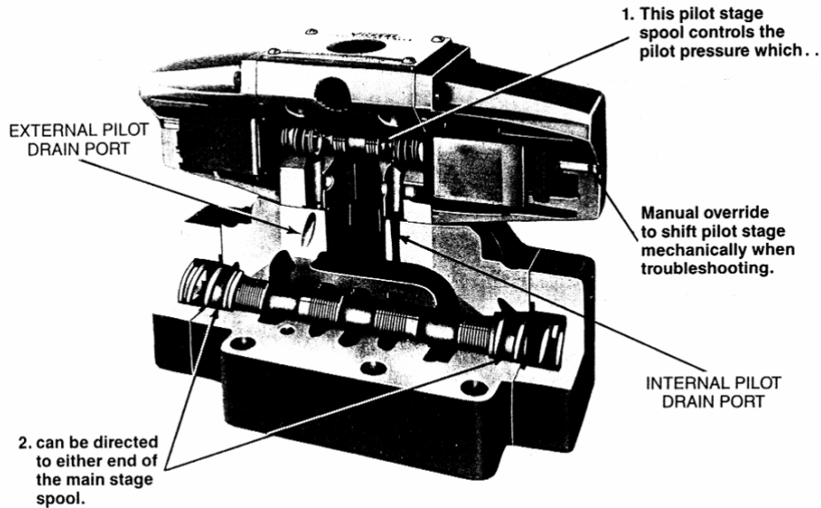
Typical solenoid-controlled, pilot-operated valve.
