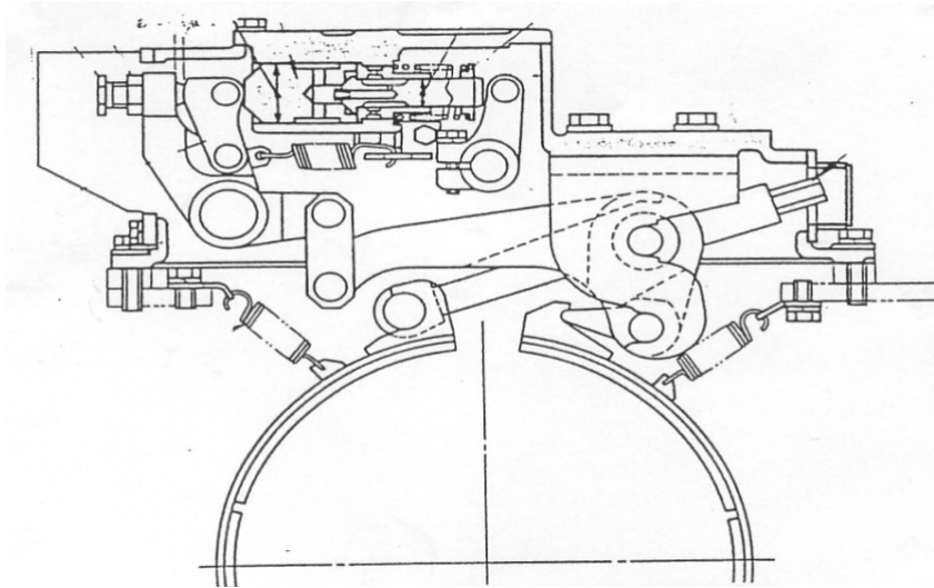
Gambar 4.119 Brake System D50, 53-17
