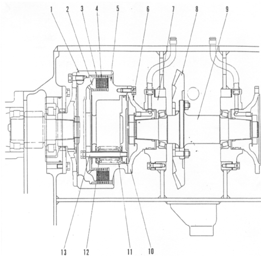
Gambar 4.115 Bevel Gear Shaft-Steering Clutch
