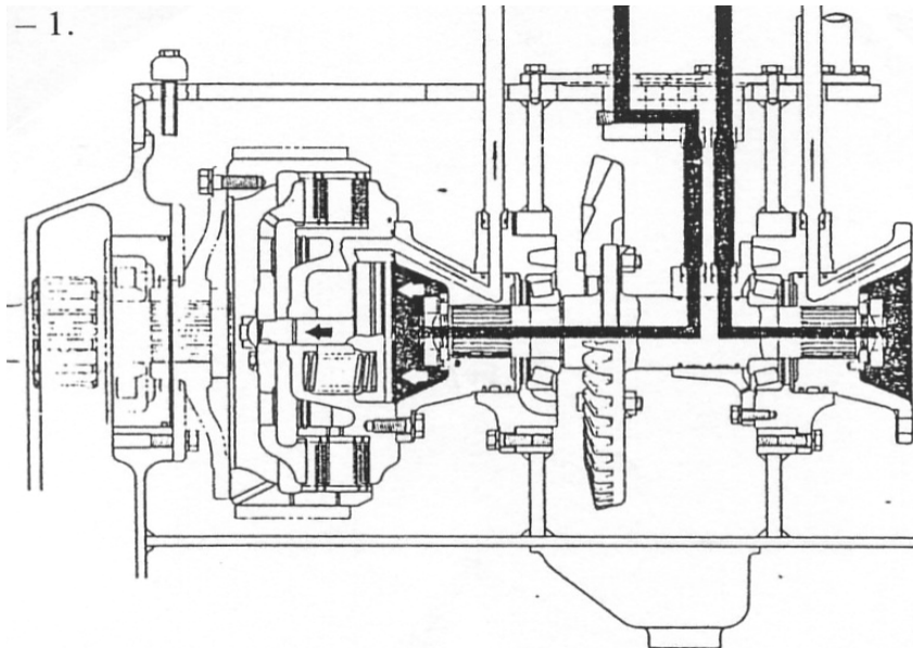
Gambar 4.134 Steering Clutch D80,85-12
