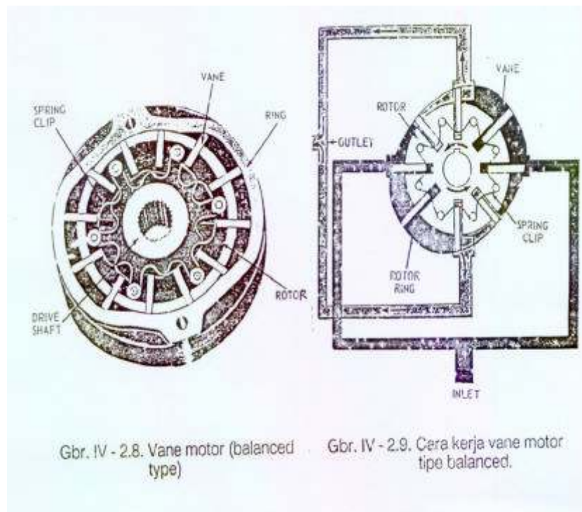
Gambar 4.158 Motor hidrolis tipe balanced
