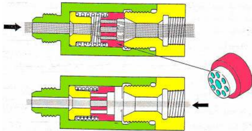
Gambar 4.113 prinsip kereja throttle valve
