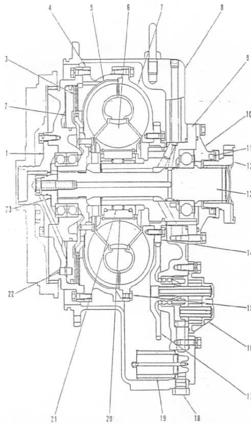
Gambar 4.182 Torque Corverter Double Phase
