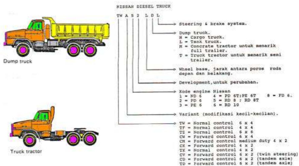
Gambar 5.42 Truck Nissan diesel
