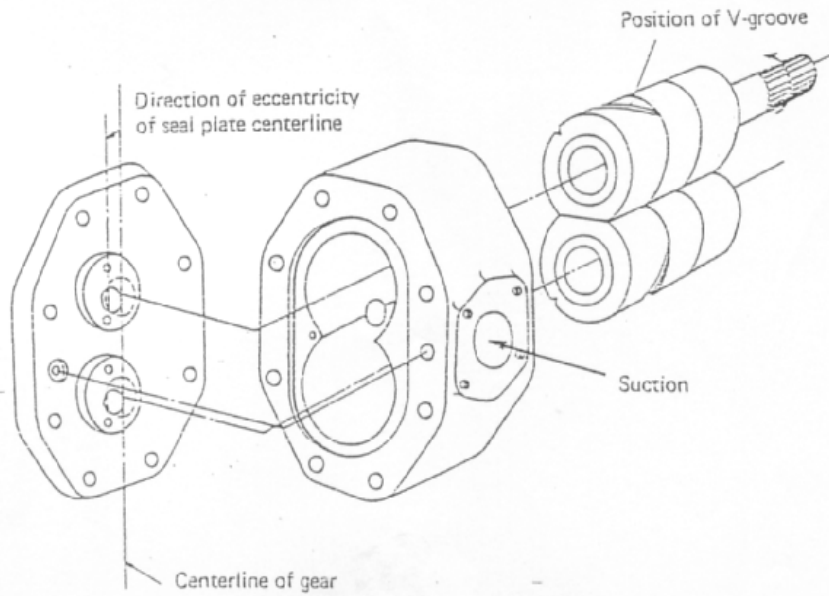
Gambar 4.73 Gear Pump tipe PAL, R014 – 025 secara Assembly Drawing
