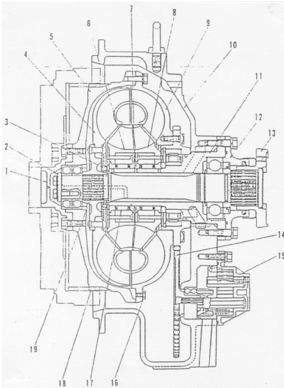
Gambar 4.183 Torque Converter Three Phase (Potongan)
