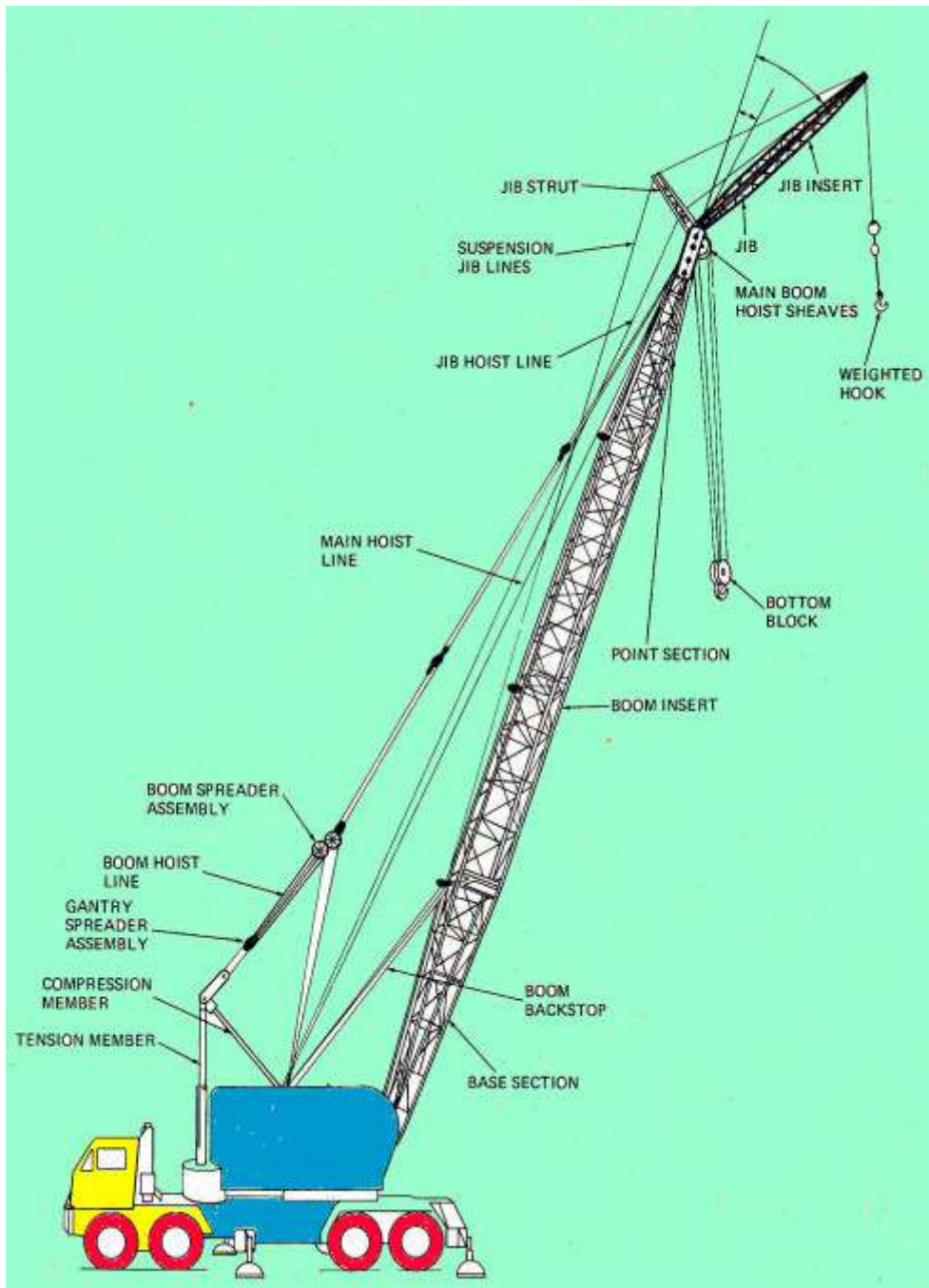
Gambar 5.3 Typical crane boom with jib attached
