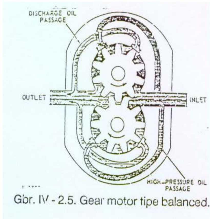
Gambar 4. 155 Motor Roda gigi tipe balanced
