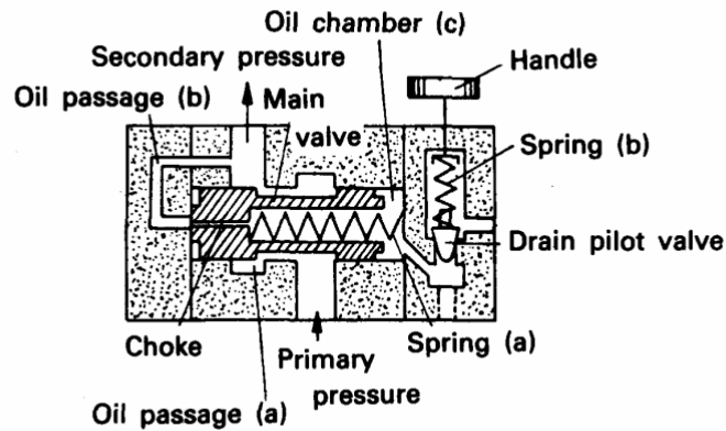
Pressure Reducing Valve Gambar 4.79 Katup Pengurang Tekanan
