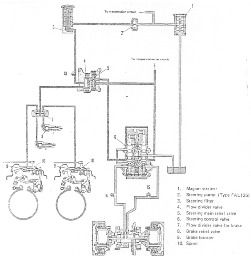
Gambar 4.132 Sirkuit Steering Clutch D355-3
