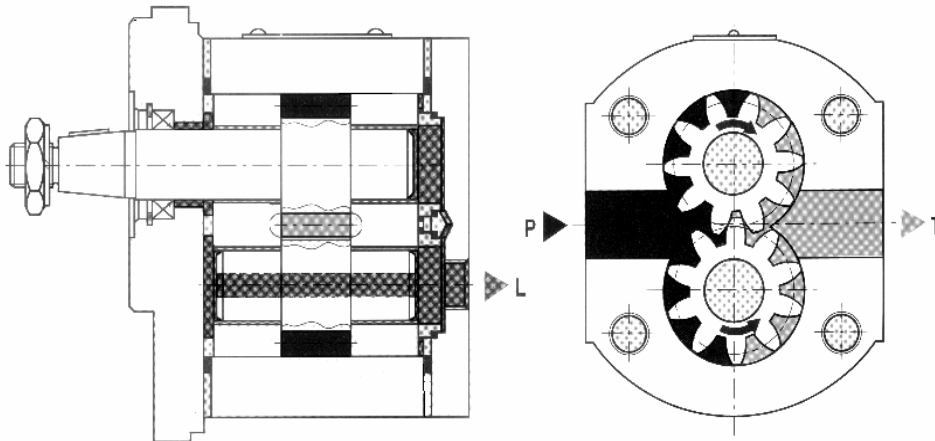
Gambar 1.7 Gear motor, type G2
