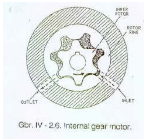
Gambar 4.156 Internal gear motor
