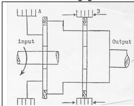
Gambar 4.202 Reverse Clutch di engage
