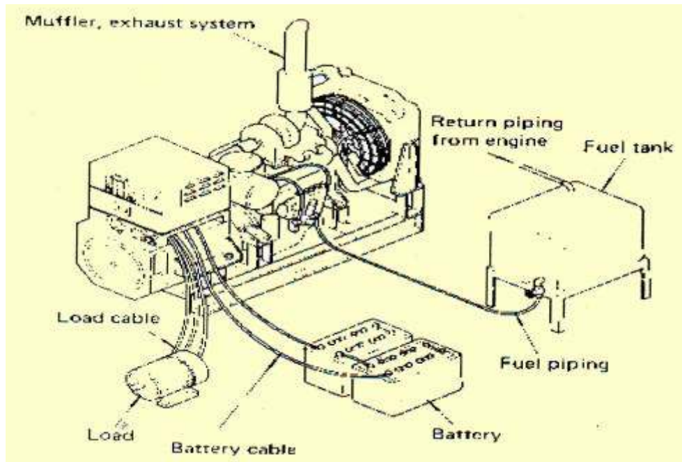
Gambar 43. Peralatan genset
