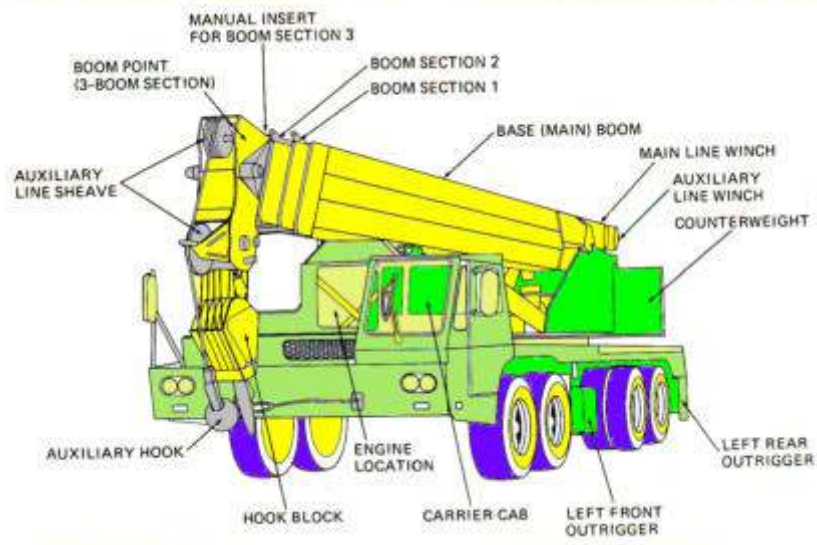
Gambar 5.2 Hydraulic motortruck crane
