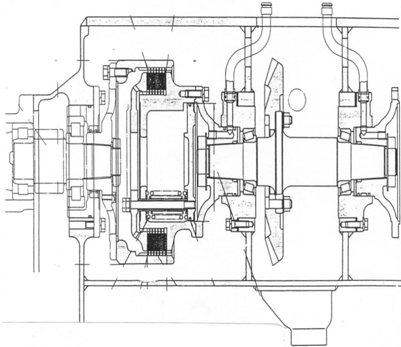
Gambar 4.124 Steering Clutch D 155-1
