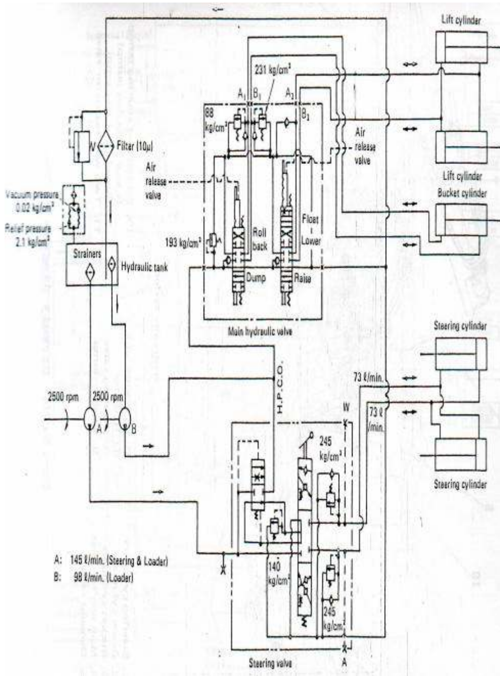
Gambar 4.122 (c) Wheel Loader W90-3
