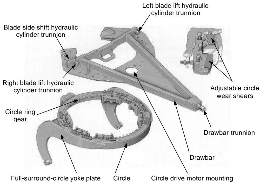
Gambar 4.157 Frame Motor grader
