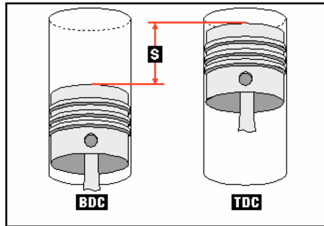
Gambar 4.3 Gambar Stroke
