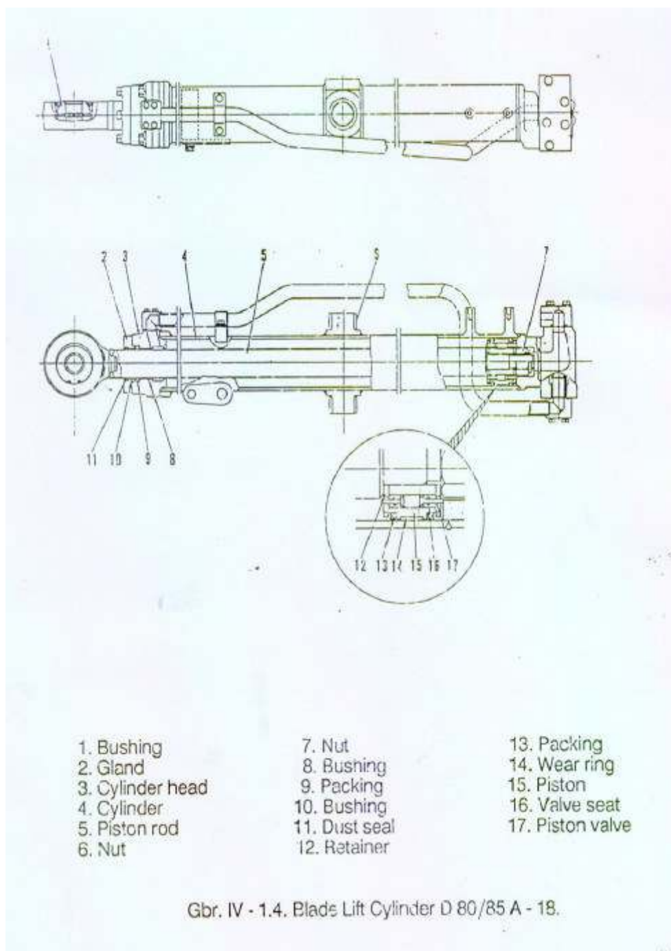
Gambar 4.148 Blade lift Cylinder D 80/85A-18
