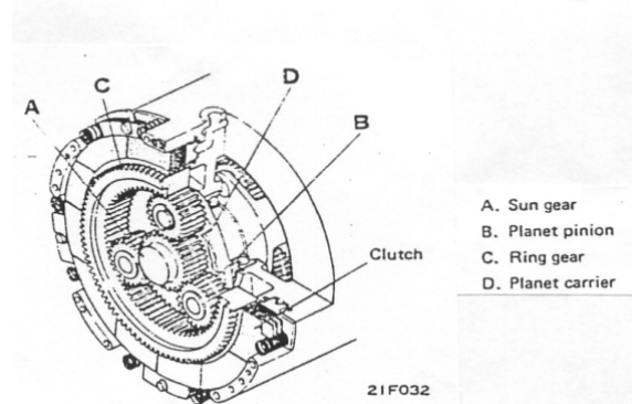
Gambar 4.198 Planetary Gear
