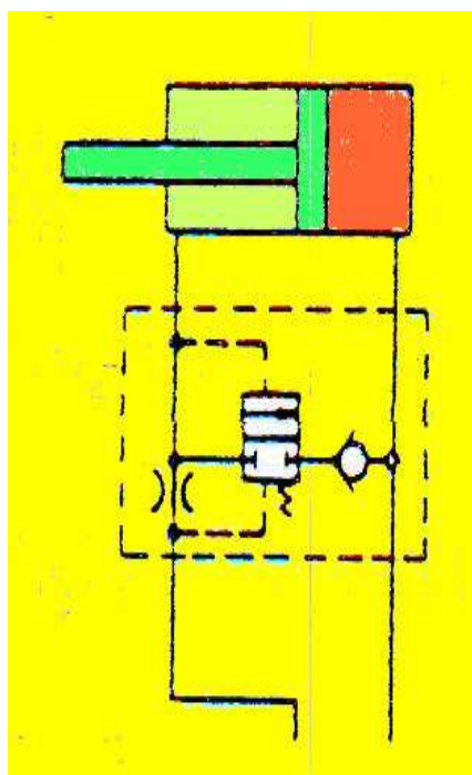
(a) (b) Gambar 4.124 Prinsip kerja quick drop valve.
