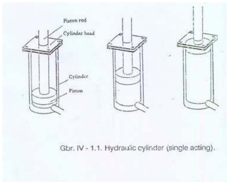
Gambar 4.145 Hydraulic cylinder (single acting)
