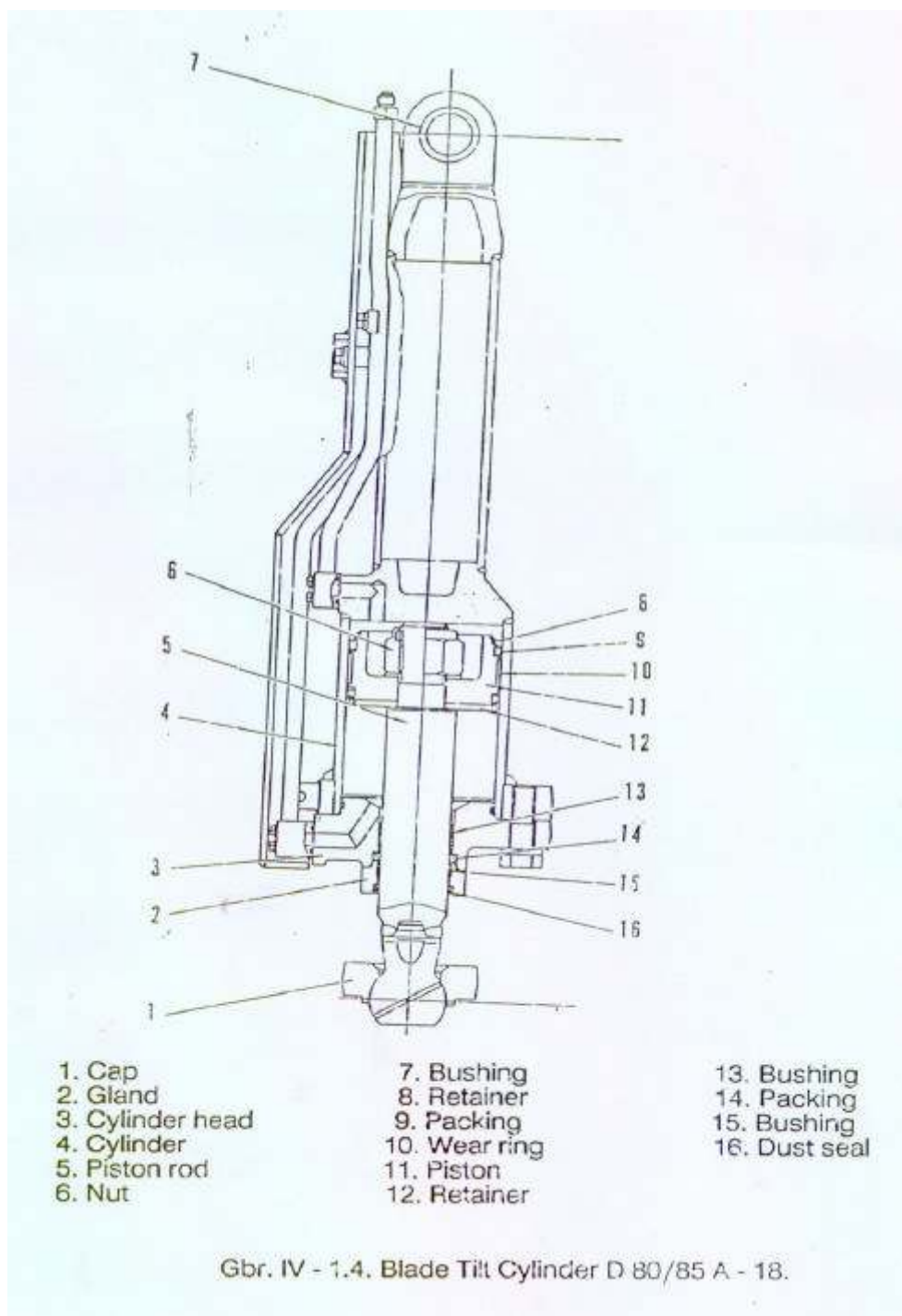
Gambar 4.149 Blade Tilt Cylinder D80/85A-18
