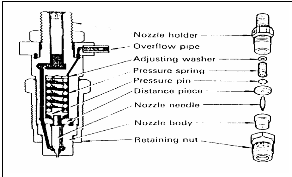
Gambar 4.46. Injection Nozzle
