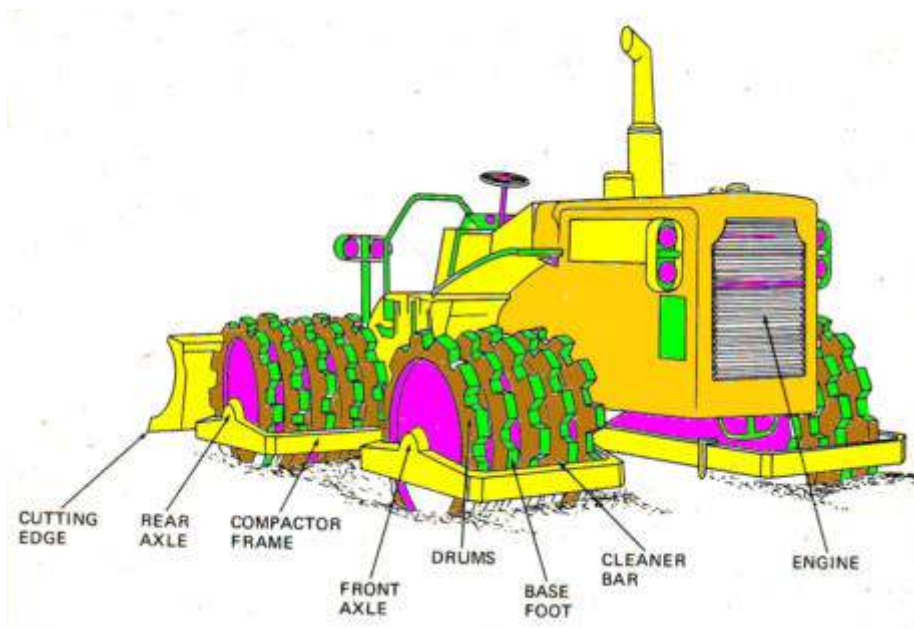
Gambar 5.42 Articulated tamping foot compactor
