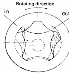
Gerotor Type Pump
