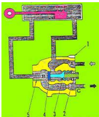
(a) (b) Gambar 4.124 Prinsip kerja quick drop valve.
