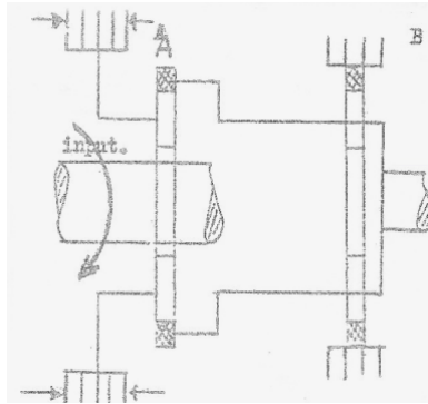
Gambar 4.202 Reverse Clutch di engage
