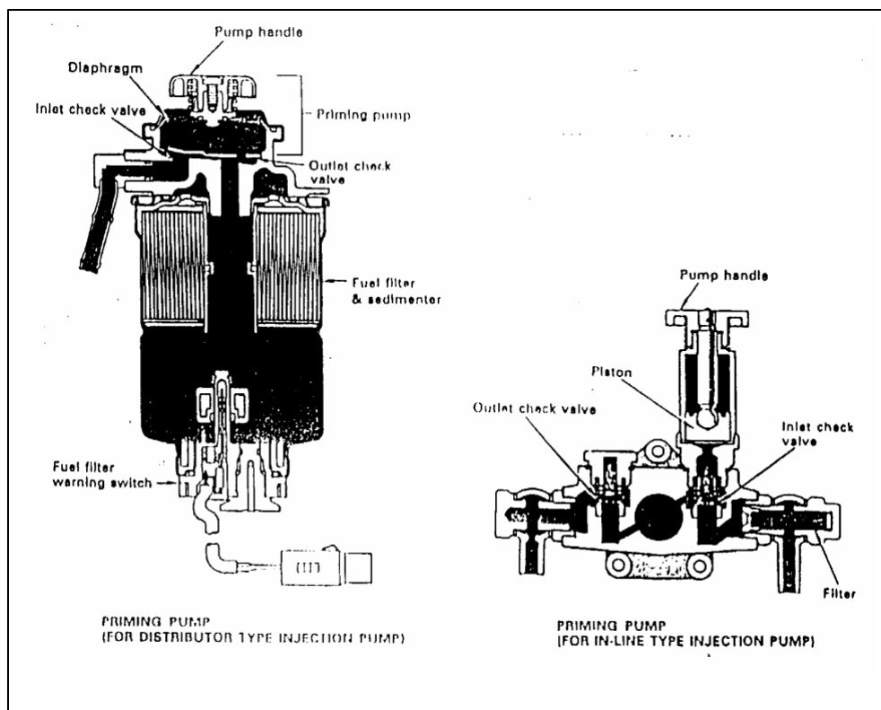
Gambar 4.42. Priming Pump
