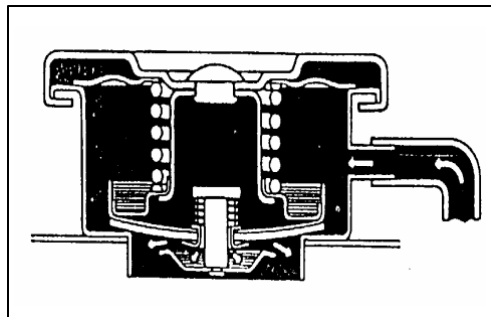
Gambar 4.23. Proses Kerja Vacuum Valve
