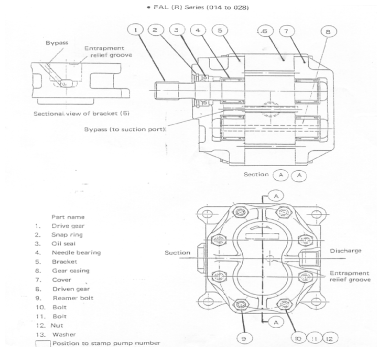
Gambar 4.72 Pressure Balancing Type Gear Pump
