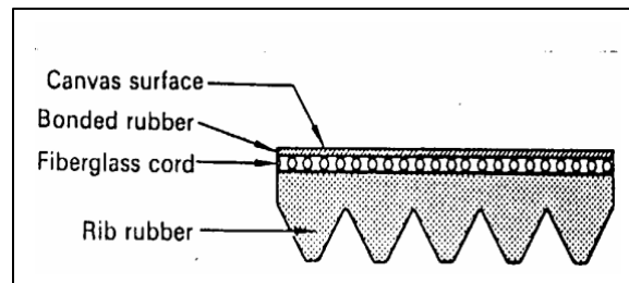
Gambar 4.30. Konstruksi V ribbed belt
