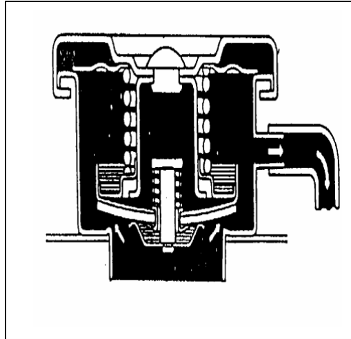
Gambar 4.22. Proses Kerja Relief Valve
