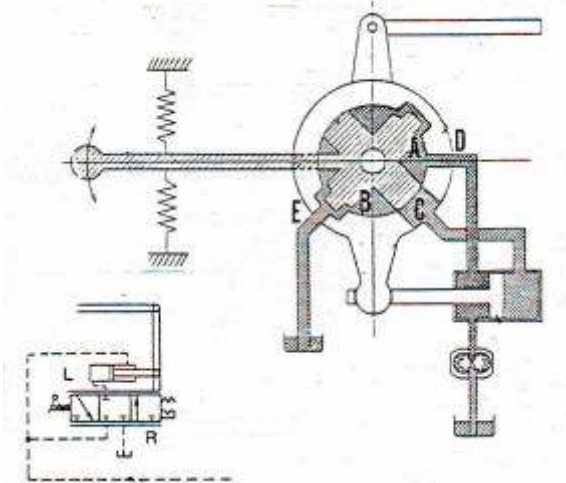
Gambar 4.134 (a) Simbol dan prinsip kerja servo rotary valve (netral)
