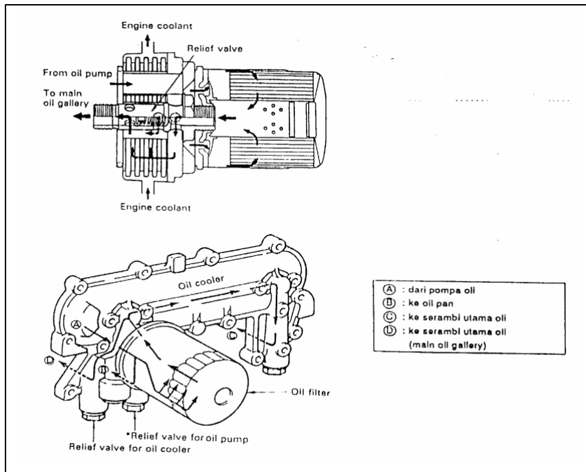
Gambar 4.38. Oil Cooler
