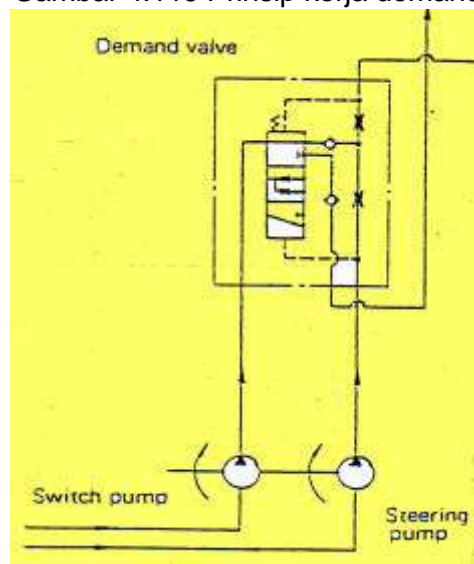
Gambar 4.120 Simbol demand valve.
