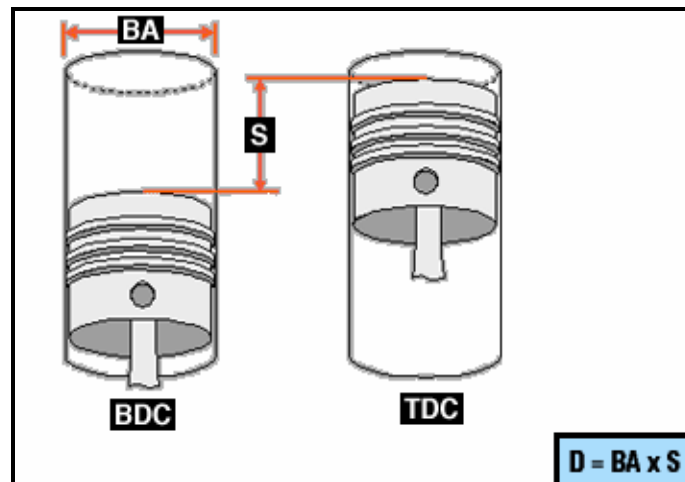
Gambar 4.4 Gambar Displacement
