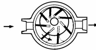
Balanced Vane Pump
