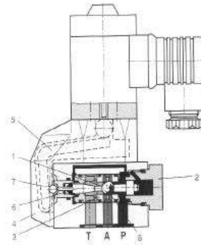
Electrically operated 3 2 way poppet valve as a single ball valve
