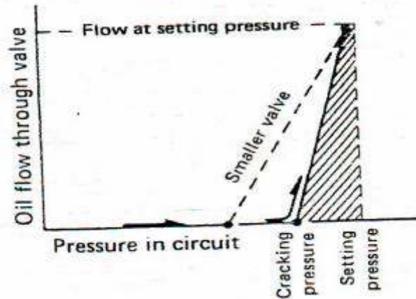
Gambar 4.111 Grafik cracking & setting pressure
