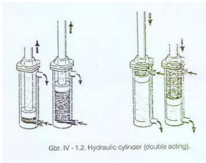
Gambar 4.146 Hydraulic cylinder (double acting)
