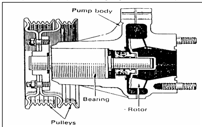
Gambar 4.25. Pompa Air ( water pump )
