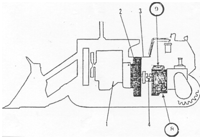
Gambar 4.194 Susunan Power Train Dozer Shovel
