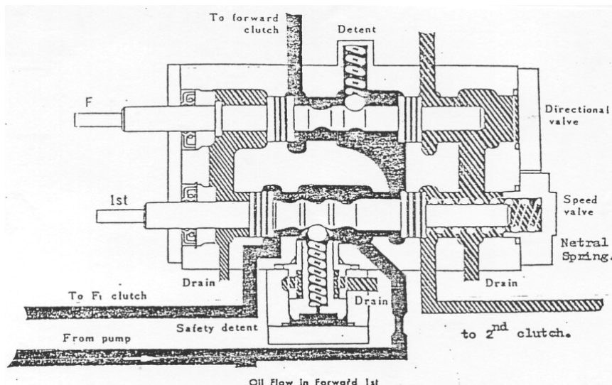
Gambar 4.212 a Control Valve type Safety Valve
