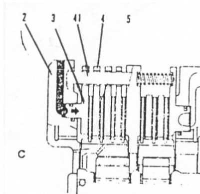
Gambar 4.204 Enggague
