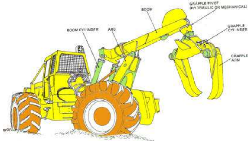
Gambar 5.30 Articulated steering skidder grapple
