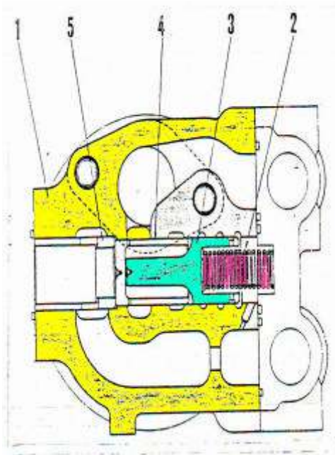
Gambar 4.123. Quick drop valve
