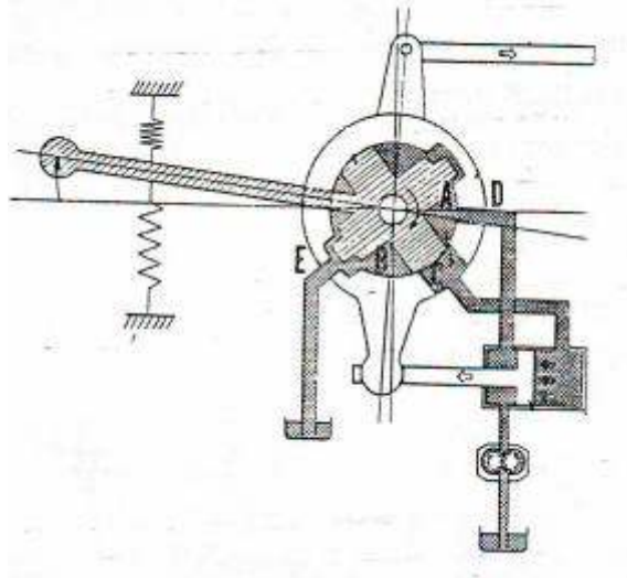
Gambar 4.134 (b) Rotary servo valve digerakkan searah jarum jam.
