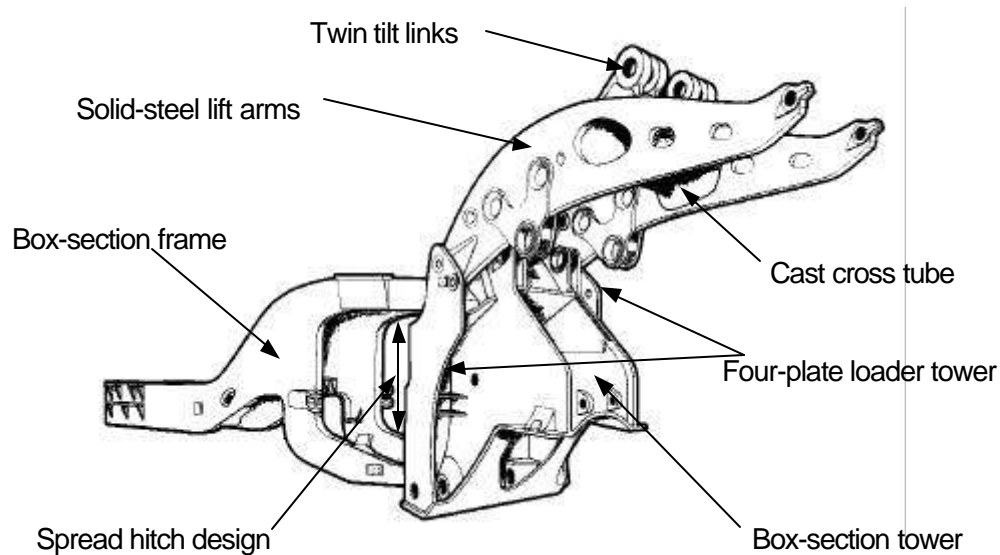
Gambar 4.153 Frame Wheel-loader
