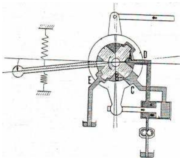
Gambar 4.134 (b) Rotary servo valve digerakkan berlawanan arah jarum jam.
