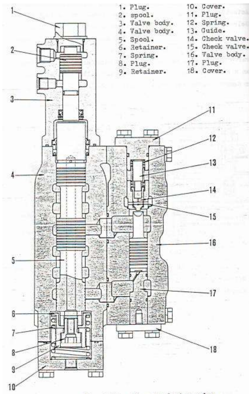
Gambar 4. 133 (c) Ripper selector valve
