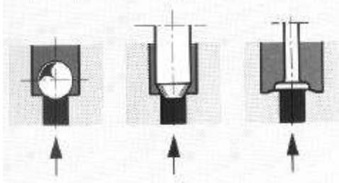
Principle of ball (left), poppet (centre) and plate seat (right)
