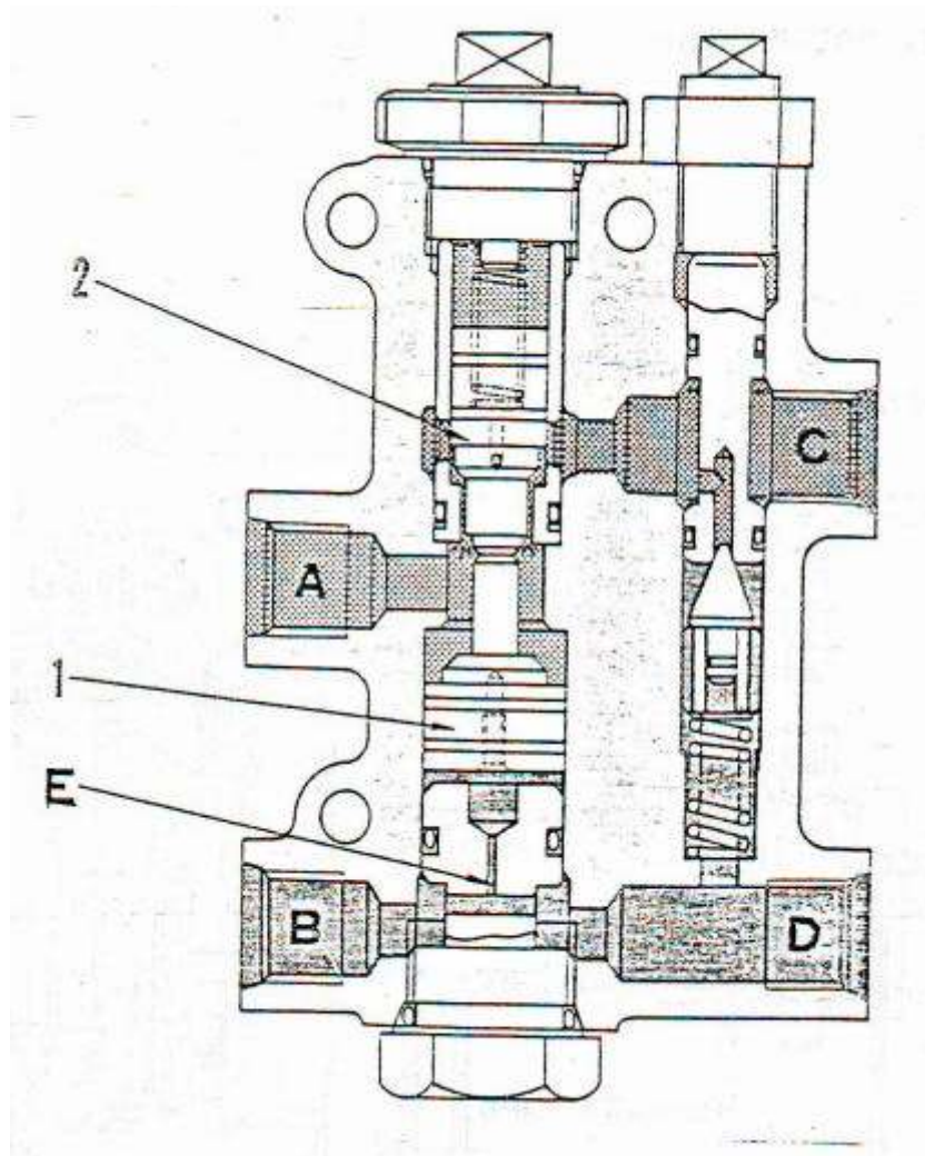
Gambar 4.132 Cara kerja pilot check valve
