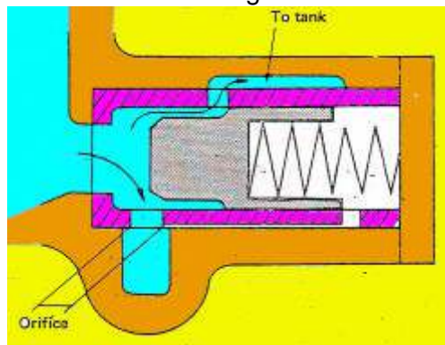
Gambar 4.116 Flow reducing valve bekerja)
