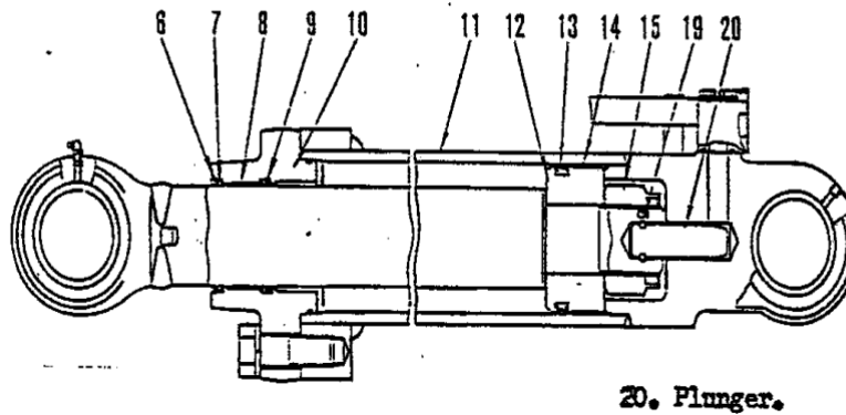
Gambar 4.141. Boom cylinder & Arm cylinder
