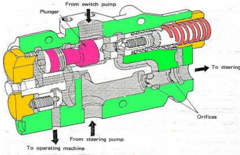
Gambar 4.119 Prinsip kerja demand valve
