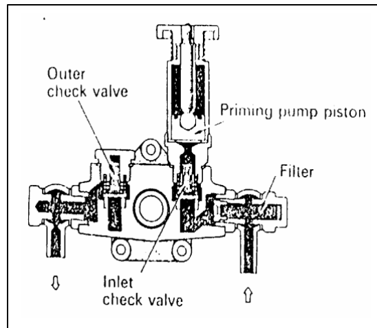
Gambar 4.43. Feed pump
